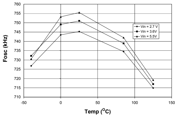
Oscillator Frequency vs Temperature Over V_{IN}
