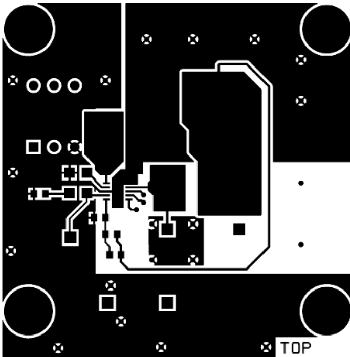
TOP COPPER
