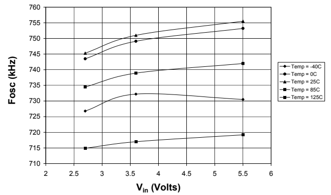
Oscillator Frequency vs V_{IN} Over Temperature
