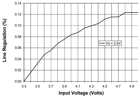
Line Regulation at I_{OUT} = 300mA
