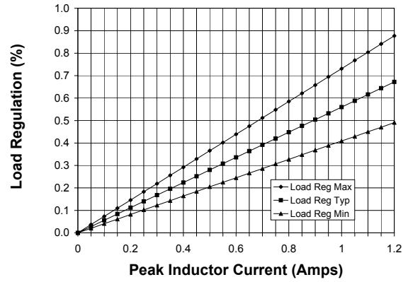
SC192 Load Regulation Limits
